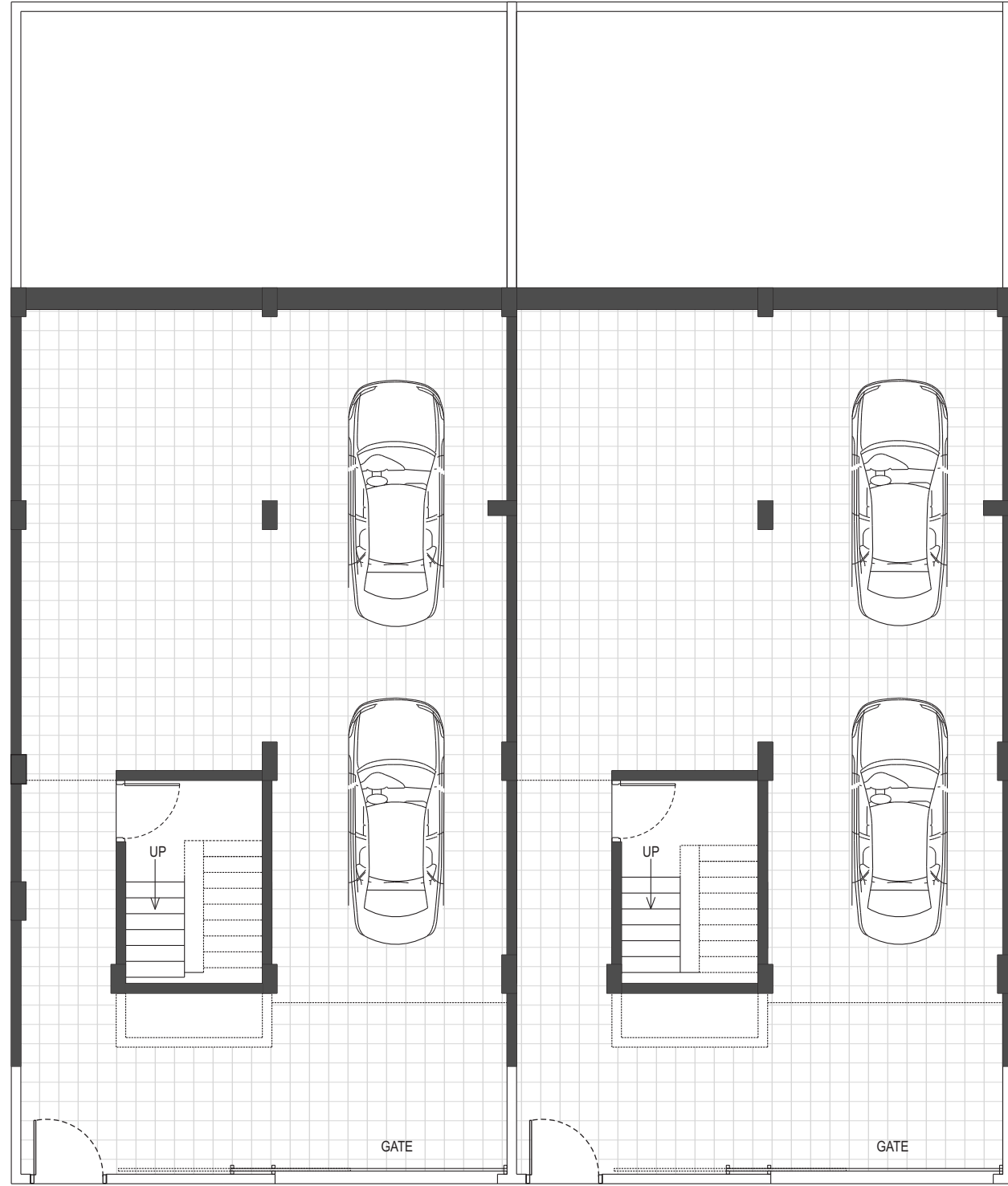
PARKING FLOOR PLAN
