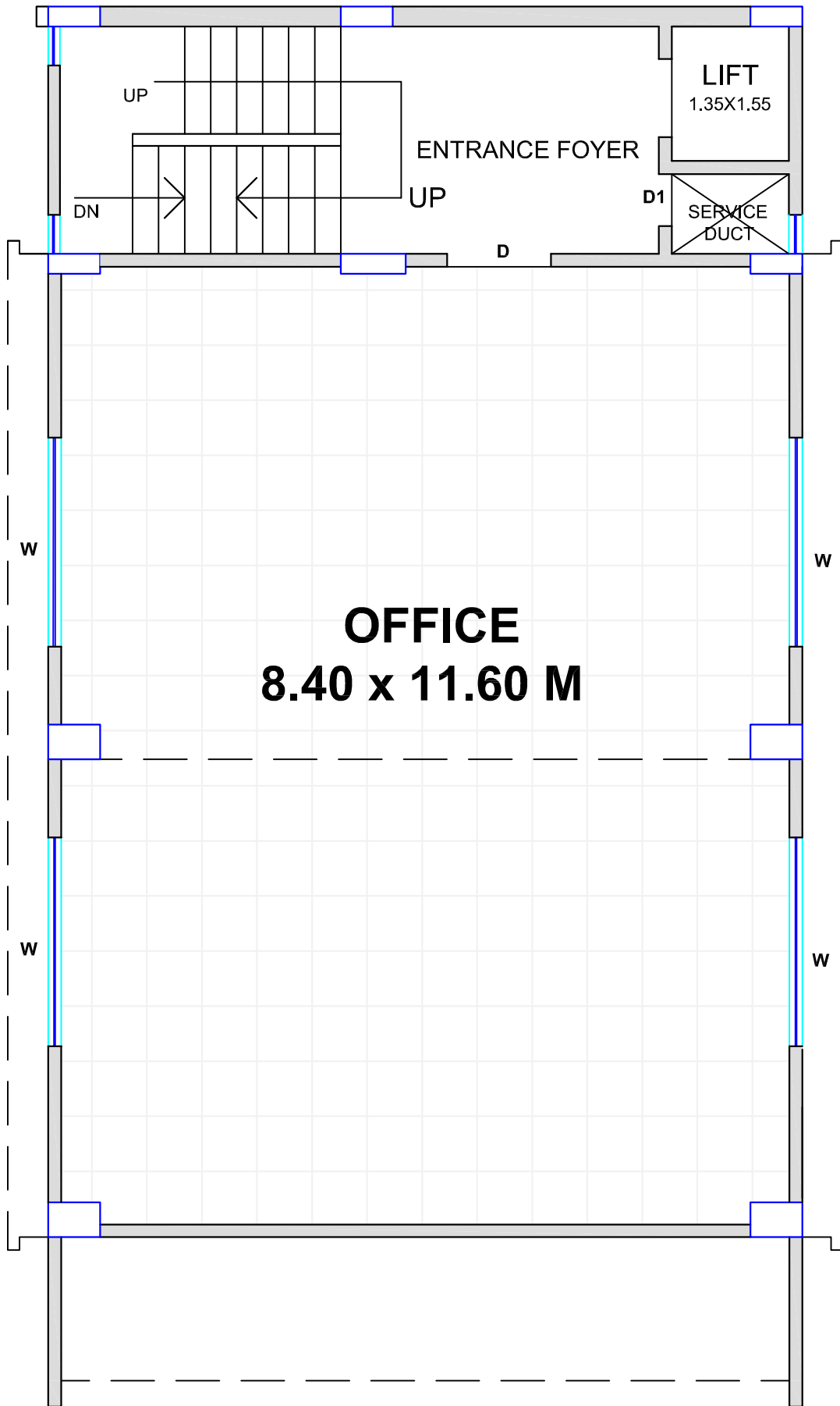
GROUND FLOOR PLAN (Double Ht.)
