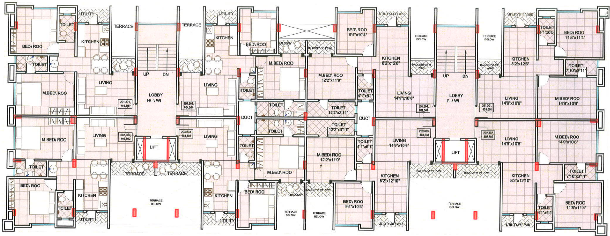
TYPICAL SECOND, THIRD, FOURTH & FIFTH FLOOR PLAN
