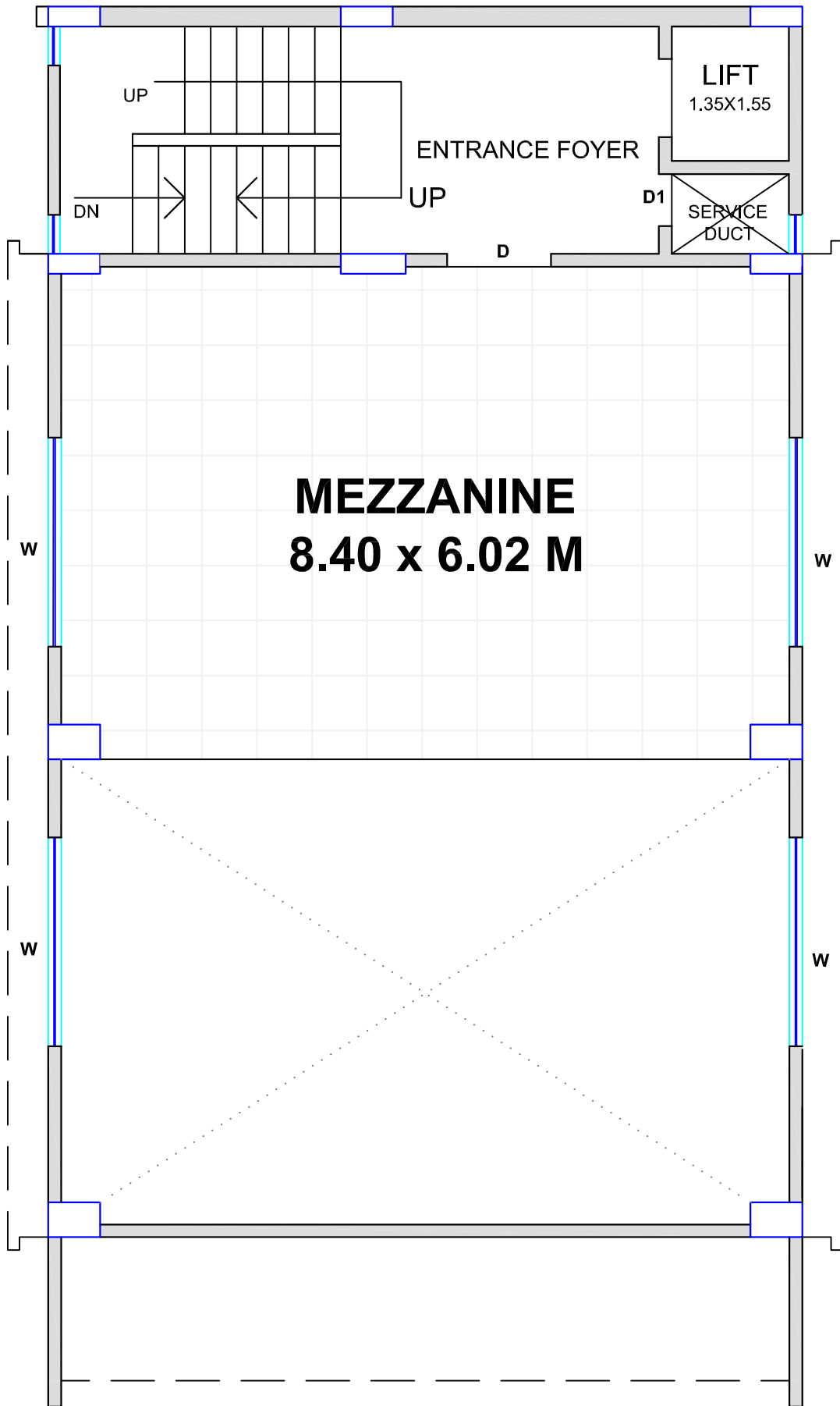
MEZZANINE FLOOR PLAN
